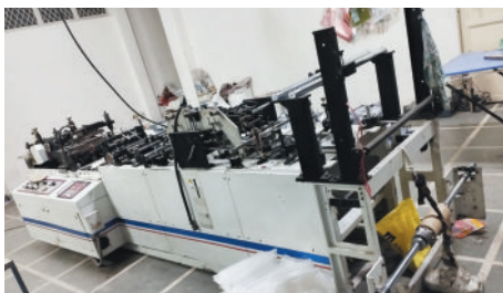
POUCHING MACHINE
